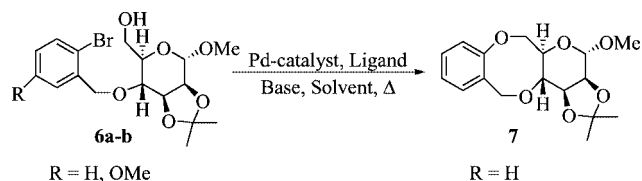
Scheme 5. Intramolecular aryl etherification of pyranose derivatives.
