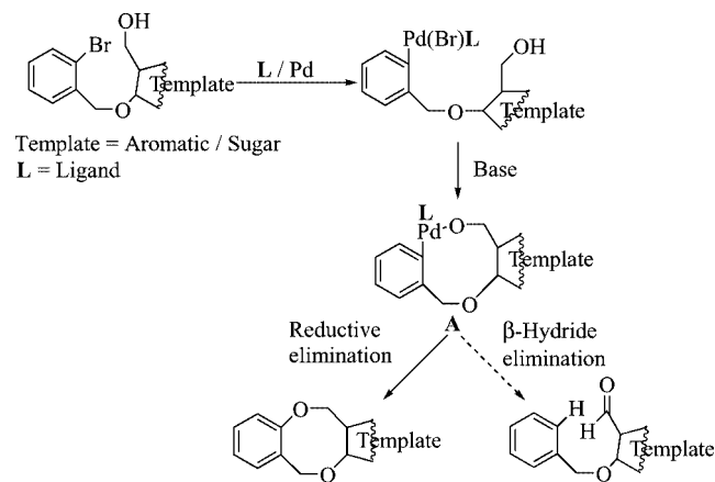
Scheme 1. Mechanism of intramolecular aryl etherification in the synthesis of medium-sized rings.
