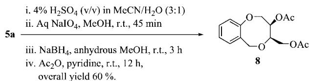
Scheme 6. Conversion of 5a to a benzodioxocine derivative.
