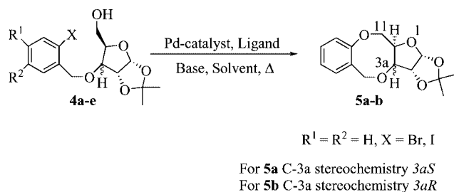
Scheme 4. Intramolecular aryl etherification of furanose derivatives.
