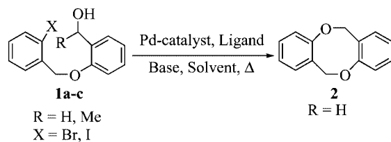
Scheme 2. Synthesis of dibenzodioxocines.
