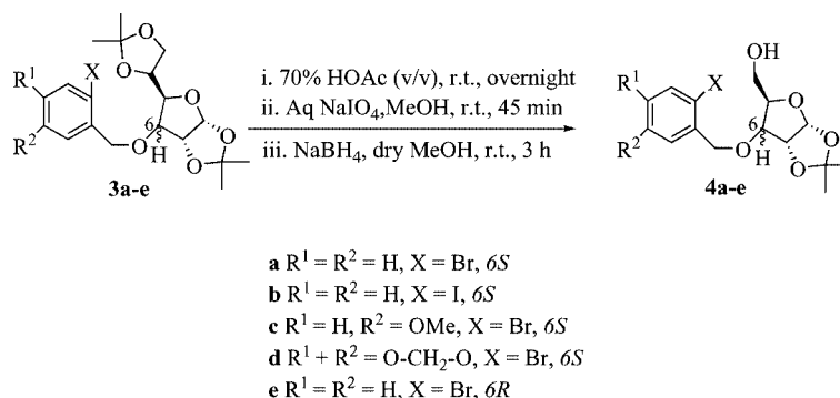
Scheme 3. Construction of O -bromo/iodobenzylated sugar alcohols.
