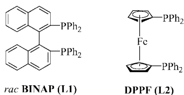
Figure 1. Ligands used in Pd-catalyzed C–O bond formation.
